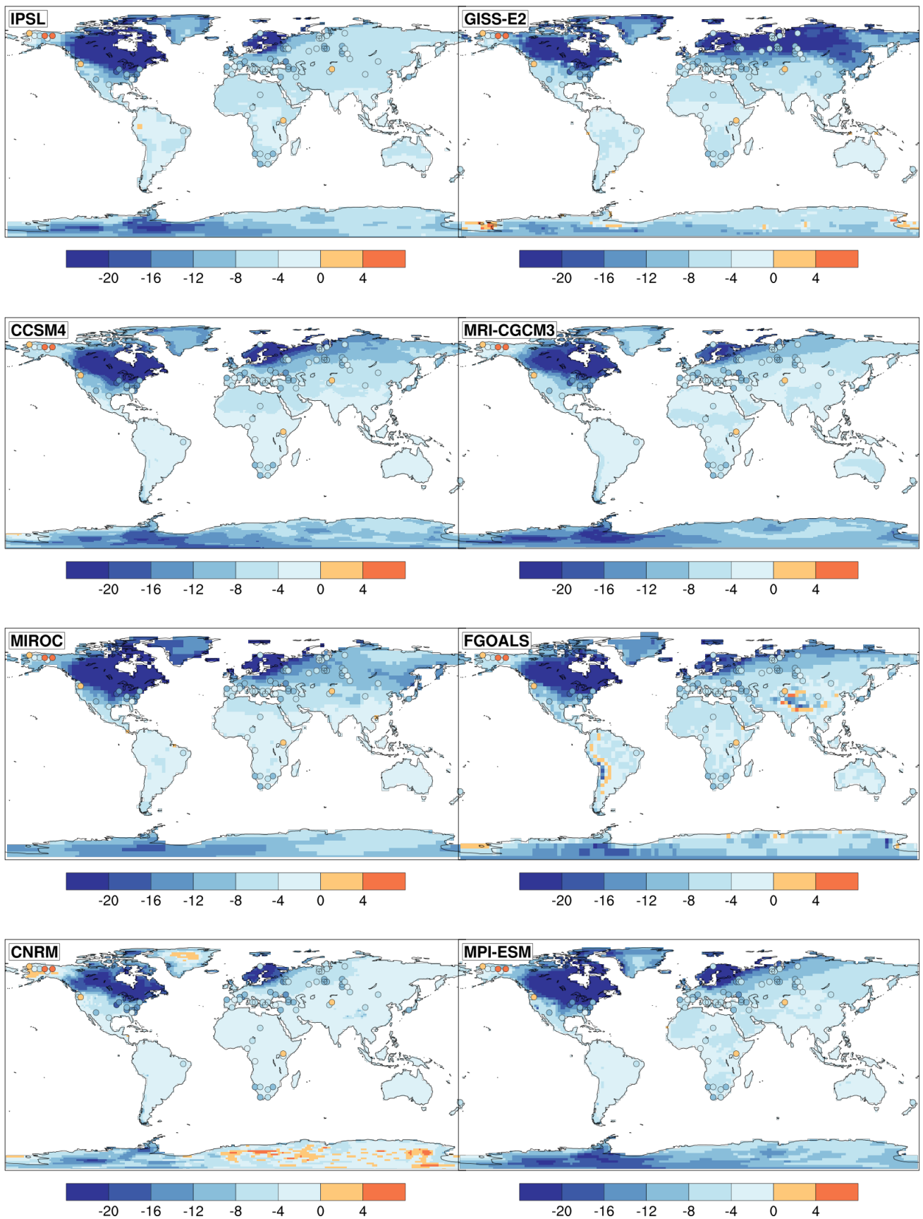
Figure 7: Background color fill: simulated global pattern of annual mean surface temperature over land ( T_{2m} ) (in ^{\circ}\text{C} ) changes between the eight PMIP3 model and PI climate. The circles localize the pollen-based reconstructed temperature changes by Bartlein et al. (2011).
