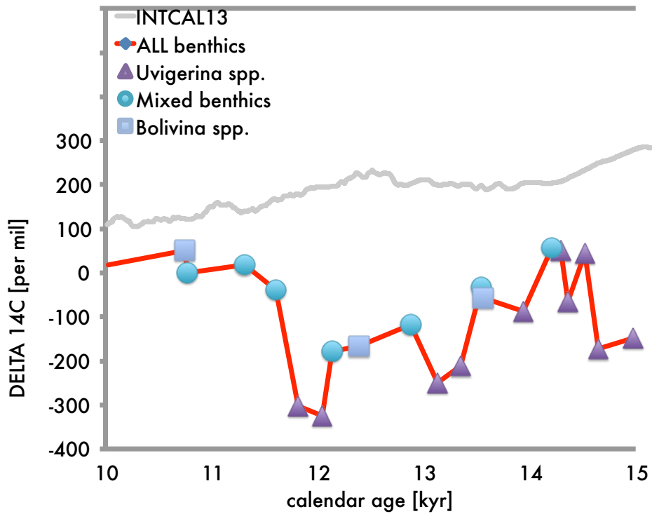
Fig. 1. Atmosphere and benthic foraminifera \Delta^{14}\text{C} (mixed, Uvi spp., and Bolivina spp.) from Marchitto et al. (2007) and Lindsay et al., (2016)
