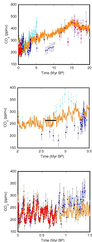
Fig. 6. Comparison of reconstructed CO 2 record with C = 39 K, with proxy records (symbols as in Fig. 3). Panel (a) for the full 20 Myr period, (b) for the period around the NH hemisphere inception and (c) for the mid-Pleistocene transition. Note that the vertical scale is different for the different panels. The horizontal bar in panel (b) indicates the onset of major glaciation in the Northern Hemisphere.
