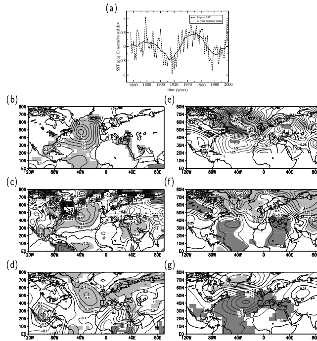
Fig. 4. (a) Index of North Atlantic SST (Kaplan et al., 1998) (dashed line) with 21-year running mean filter (solid line). Difference between warm phase 1940–1960 and cold phase 1970–1990 of North Atlantic (b) SST (Kaplan et al., 1998) and (e) SLP (Trenberth and Paolino, 1980) from observational data, ensemble mean of ECHAM simulations for (c) SAT and (f) SLP, and ensemble mean of PUMA simulations for (d) SAT and (g) SLP. Units are given in °C and hPa. Contour interval is 0.1°C and 0.25 hPa. Shading indicates significance at 95% confidence level, according to a t-test statistics.
