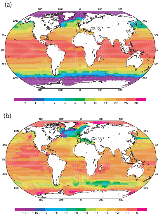
Fig. 7. (a) Sea Surface Temperatures at the LGM (°C) (b) LGM-LH_CTRL Sea Surface Temperature differences (°C). Both panels are averages over the last 200 years of the simulations.
