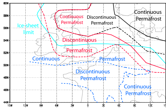
Fig. 5. Permafrost in western Europe: data and model. Limits of permafrost are outlined as follow: continuous black line (respectively dashed black line) is the continuous (respectively non-continuous) permafrost limit for the simulated LGM, continuous red line (resp. dashed red line) is the continuous (resp. non-continuous) permafrost limit for the “continentiality” sensitivity experiment (see text) and continuous dark blue line (resp. dashed dark blue line) is the continuous (respectively non-continuous) permafrost limit inferred from the data (Renssen and Vandenberghe, 2003). The continuous light blue line is the limit of the imposed ice-sheet in the atmospheric part of the model.
