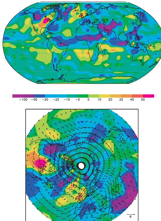
Fig. 2. Changes in simulated precipitation at the LGM with respect to the LH_CTRL (in mm.yr -1 ). Panel a shows the precipitation anomaly (LGM-LH) over the globe. Panel b shows the precipitation anomaly (LGM-LH) for the northern hemisphere, with LGM to LH_CTRL changes in the wind field superimposed as vectors. All panels show averages over the 200 last years of the simulations.
