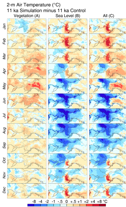
Figure 9. The effect on 2 m air temperature (°C) of changing vegetation (a), sea level (b) and all three land cover changes (vegetation, sea level and lakes; c) at 11 ka. Ice-sheet and coastal outlines as in Fig. 4.
