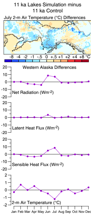
Figure 8. Results of 11 ka Lakes experiment. Top panel shows July 2 m air temperature differences (11 ka Lakes minus 11 ka Control). Lower panels show mean monthly differences for energy fluxes and temperature for RegCM grid cells in western Alaska (170–150° W longitude), where cooling is most pronounced. Ice-sheet and coastal outlines as in Fig. 4.
