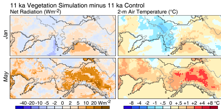
Figure 7. Results of 11 ka Vegetation experiment (11 ka Vegetation minus 11 ka Control). Panels show net radiation (left) and 2 m air temperature (right) for January (upper) and May (lower). The effect of taller, denser shrub/tree cover is seen most strongly in May, when 2 m air temperatures increase by 1–4 °C over the control values. Ice-sheet and coastal outlines as in Fig. 4.
