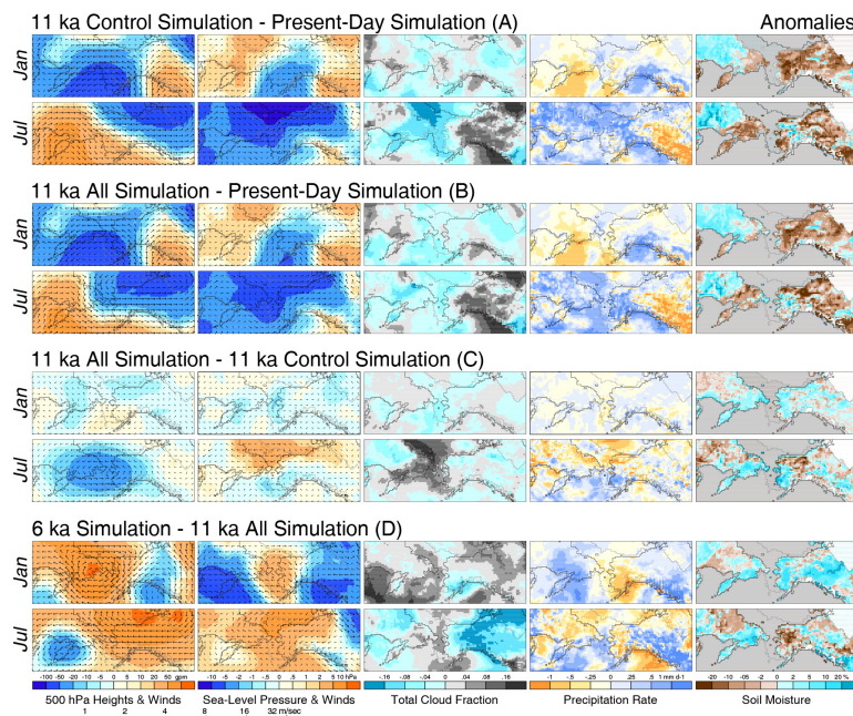
Figure 10. Atmospheric circulation (500 hPa heights and winds, sea-level pressure and surface winds), clouds, precipitation and soil-moisture anomalies. (a) 11 ka Control minus Present Day; (b) 11 ka All minus Present Day; (c) 11 ka All minus 11 ka Control; (d) 6 ka minus 11 ka All (showing the change between 11 and 6 ka). Ice-sheet and coastal outlines as in Fig. 4.
