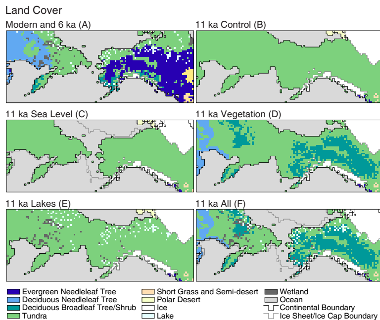
Figure 4. Land cover for RegCM climate simulations. Modern conditions are also used for the 6 ka simulation; there are minor differences in forest cover between modern and 6 ka (see Fig. 3). The vegetation cover in each simulation is represented by the set of RegCM plant functional types (PFTs); the PFT Deciduous Broadleaf Tree/Shrub was created to represent the characteristics of short-statured deciduous woodland and tall shrub communities. Land cover for 11 ka All ( f ) combines all three experimental land-cover changes. Each land-cover map is linked to a RegCM simulation; an additional simulation was made using modern land cover with 11-ka continental outlines (not shown).
