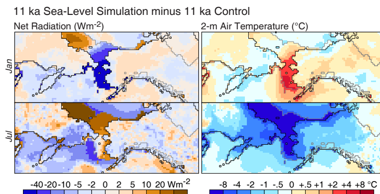
Figure 6. Results of 11 ka Sea Level experiment. Panels show the effect of flooding the land bridge at 11 ka (11 ka Sea Level minus 11 ka Control). Net radiation (left) and 2 m air temperature (right) for January (upper) and July (lower). Strong winter warming and summer cooling is seen over areas of flooded ocean shelf and adjacent land areas. Ice-sheet and coastal outlines as in Fig. 4.
