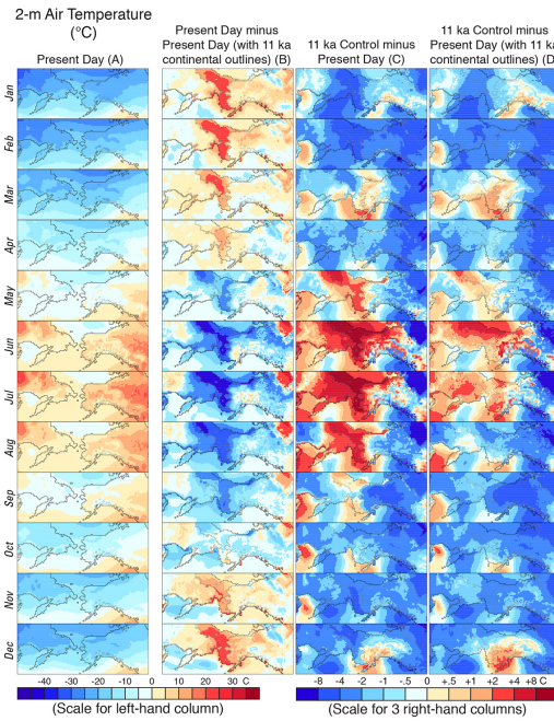
Figure 5. Simulated 2 m air temperature. (a) Present-Day (0 ka) simulation; (b) effect of land bridge flooding on present day climatology (Present Day minus Present Day with 11 ka continental outlines); (c) difference between 11 ka Control and present (11 ka Control minus Present Day); (d) difference between 11 ka Control and present as a result of insolation and boundary conditions other than sea level (11 ka Control minus Present Day with 11 ka continental outlines). Ice-sheet and coastal outlines as in Fig. 4.
