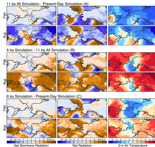
Figure 12. Net shortwave radiation (surface), net radiation and 2 m air temperature differences for February and August. (a) 11 ka All minus Present Day, illustrating the impact of 11 ka insolation (relative to that at present); (b) 6 ka minus 11 ka All, illustrating the impact of changes in boundary conditions other than concurrent insolation between 11 and 6 ka; (c) 6 ka minus Present Day, illustrating the impact of 6 ka insolation (relative to that at present). Ice-sheet and coastal outlines as in Fig. 4.
