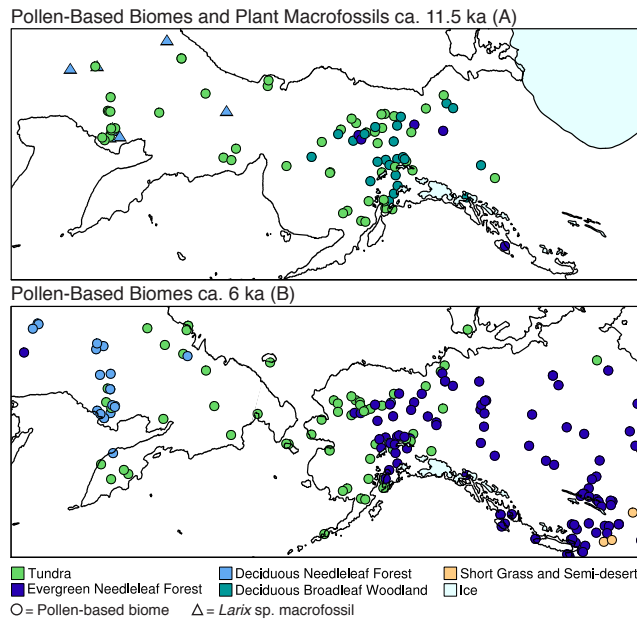
Figure 3. Pollen-based biomes for ca. 11.5 ka ( a ; this study) and ca. 6 ka ( b ; from Prentice et al., 2000; Bigelow et al., 2003). The 11.5-ka pollen patterns indicate deciduous broadleaf woodland in Alaska and Canada ( a ), but in Siberia this biome is identified from macrofossils only (not shown; see Sect. 2.2.8). At 6 ka deciduous needleleaf forest in Siberia is identified from widespread Larix pollen. The main difference between 6 ka and modern is the truncated distribution of evergreen needleleaf forest in western Alaska at 6 ka. Biome identities and colours map on to the RegCM land-cover PFTs in Fig. 4. Ice from Dyke et al. (2003) and coastline inferred from Peltier (1994) topographic anomalies.
