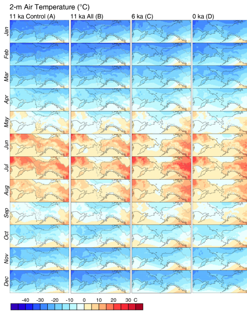
Figure 11. Monthly mean simulated temperature for 11 ka Control ( a ), 11 ka with changed surface properties (11 ka All; b ), 6 ka ( c ), and present (0 ka; d ). Ice-sheet and coastal outlines as in Fig. 4.
